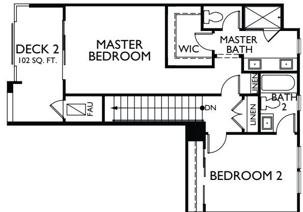
THIRD FLOOR
