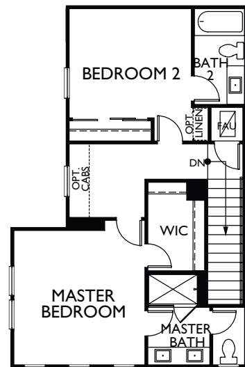
THIRD FLOOR
